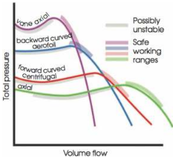
Fan Performance Curve
