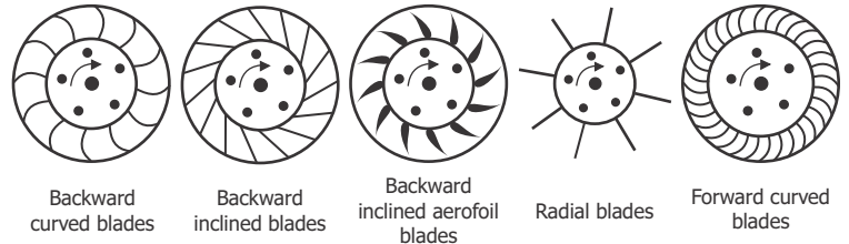
FIG E. High Pressure Blower Impeller can be used with directly mounted on shaft and motor shaft. This type of Blower generally used with high pressure and low volume of air in Melting Furnace, Induced draft type, Dust Collector Bag filter, Exhaust of Air etc.
